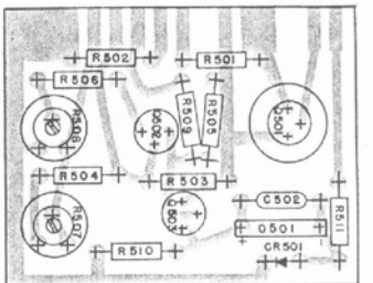
Deviation Amplifier 1P84305A02
