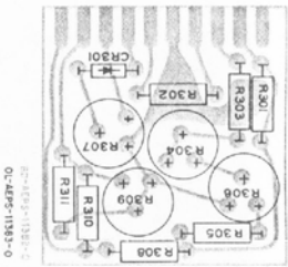
Increment Adjust 1P83554F01
