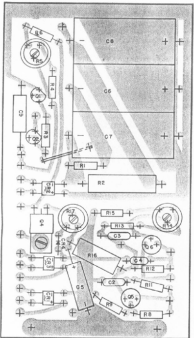
Power Supply 1P84305A07
