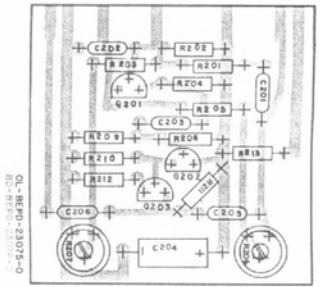
Audio Oscillator 1P84305A03
