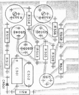
Deviation Amplifier 1P84305A02
