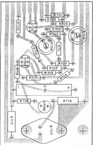
Deviation Amplifier 1P84207D63
